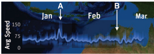
Figure 3: Speed timeline shows the average speed profile of each selected species, in this case, the Blue Whale. The faded banding represents the minimum and maximum within the species. Points A and B are used in an example described in Section 3.3.
